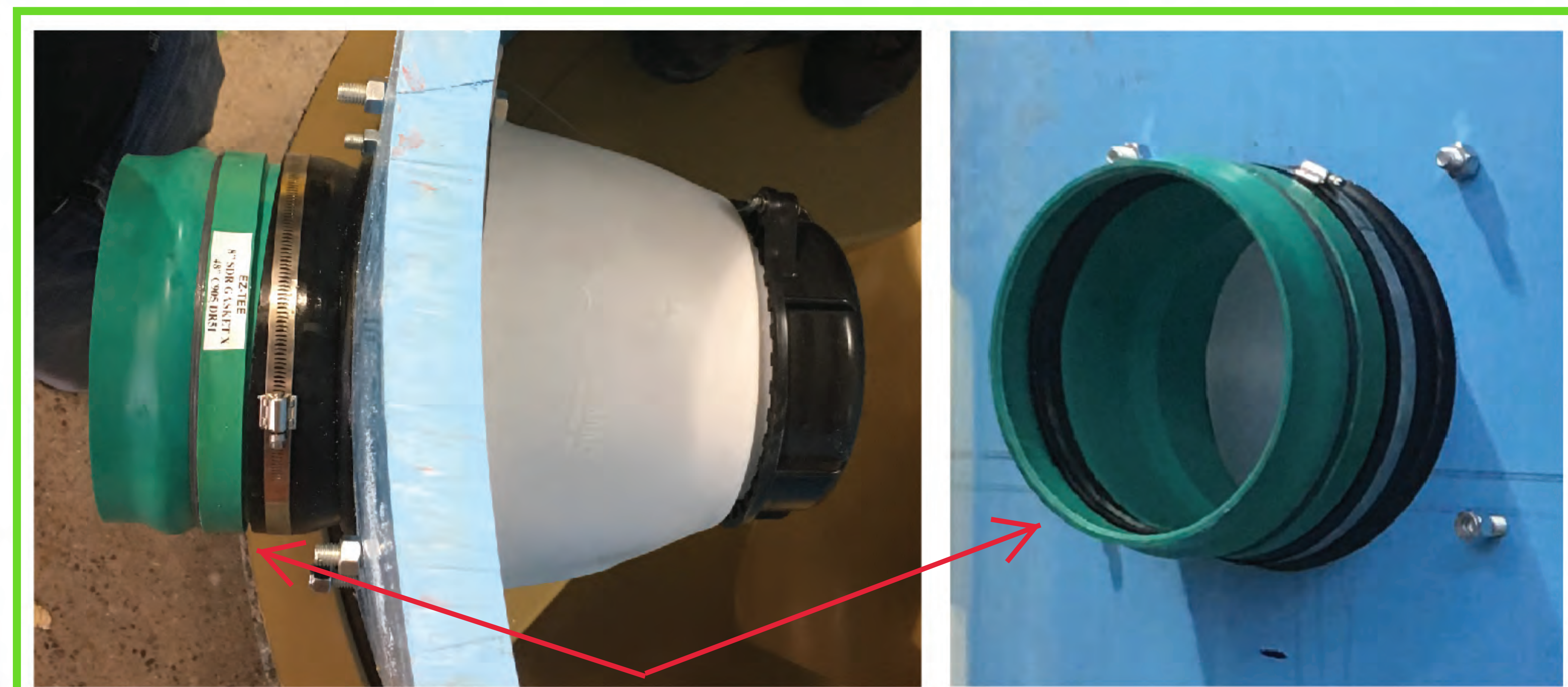
ASTM F477 COMPLIANT CLEAN OUT CONNECTION FOR OUTSIDE DROP
